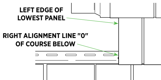
TRIPLE 5"
